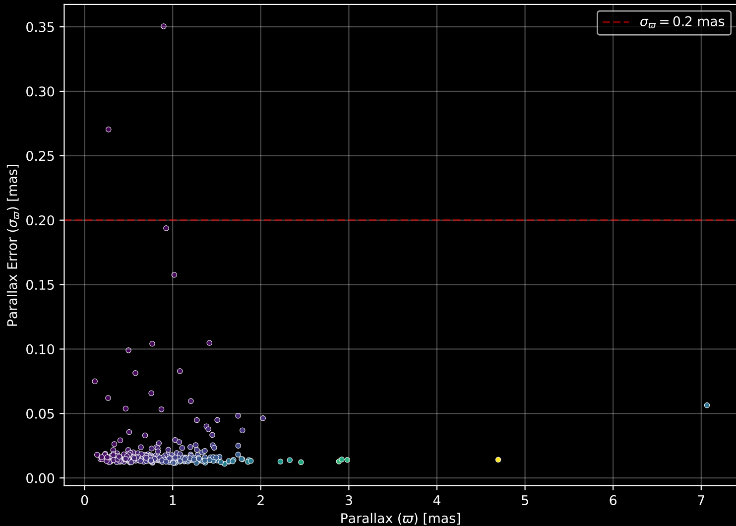
GALAH DR4 Field: [8753] Parallax Quality (n= 277)
