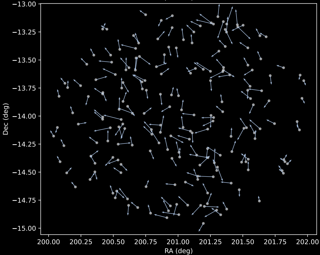
GALAH DR4 Cluster 1 Proper Motion Vectors (n=198)
