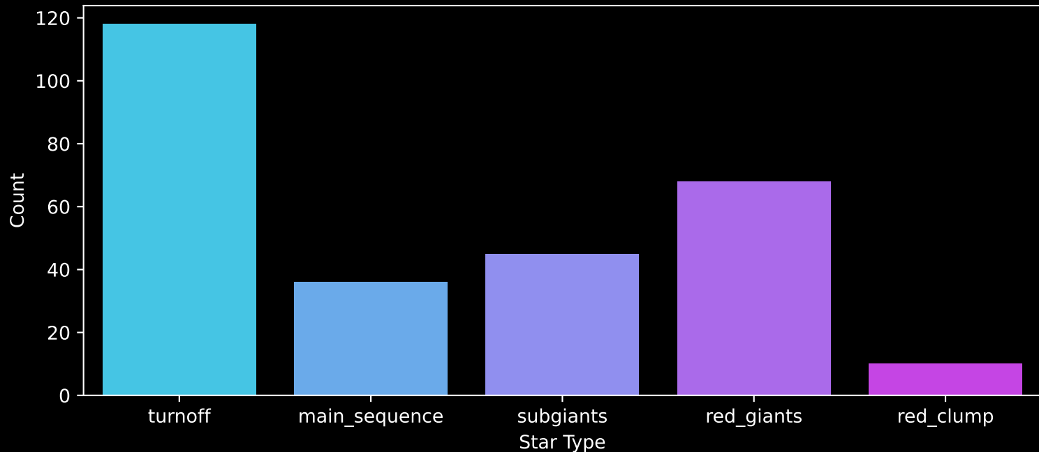
GALAH DR4 Field: [8753] Count plot of Star Type
