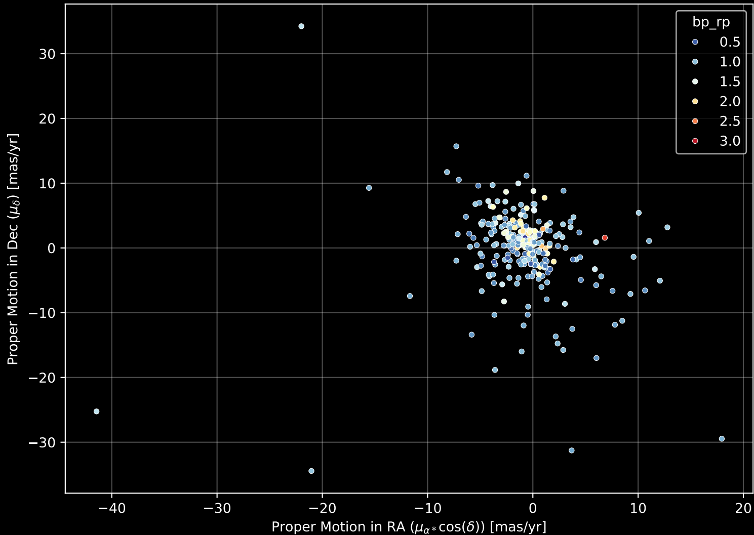
GALAH DR4 Field: [8753] Proper Motion Diagram (n= 277)
