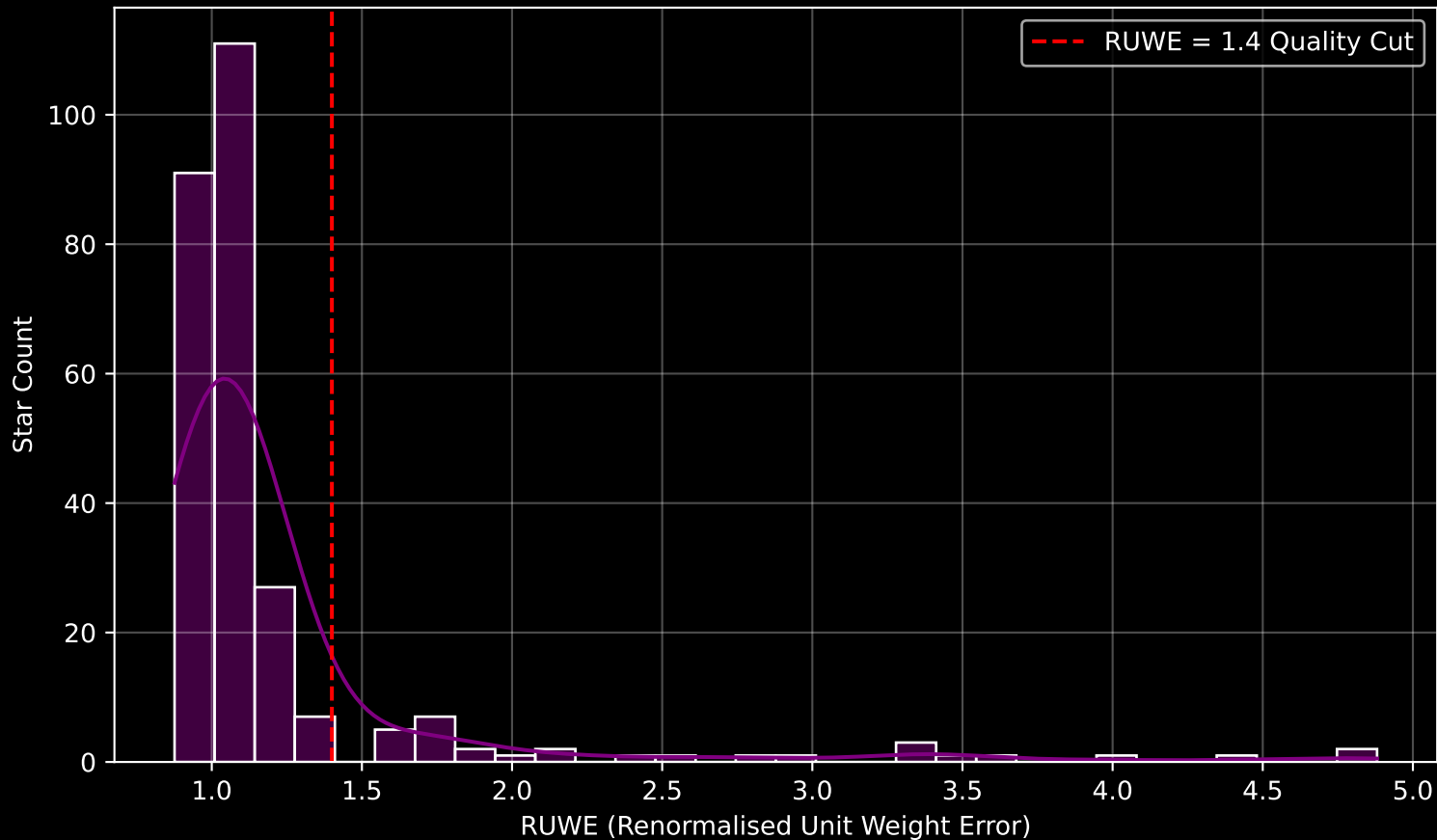
GALAH DR4 Field [8753] RUWE Distribution (n= 266)
